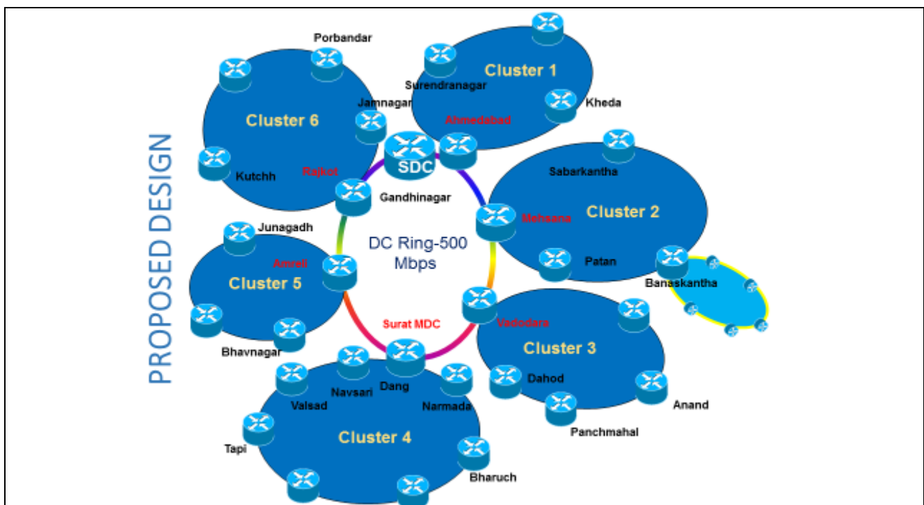
Fig 2. New Topology
